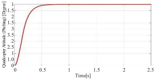
FIG. 5. PITCH RESPONSE
