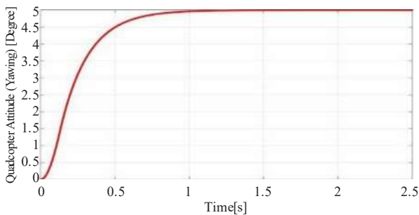
FIG. 6. YAW RESPONSE
