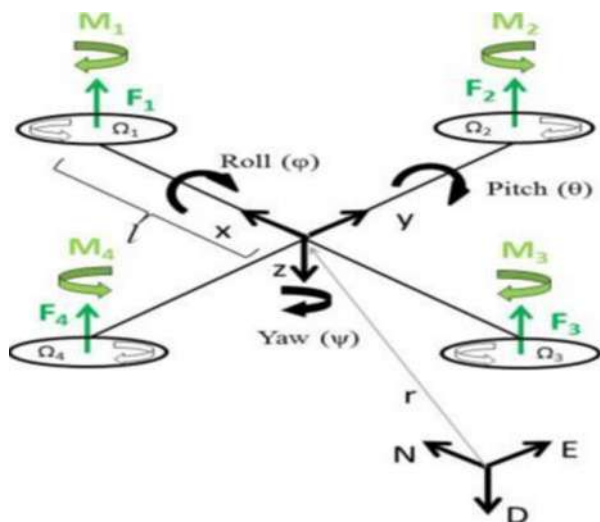
FIG. 1. SCHEMATIC DIAGRAM OF A QUADCOPTER
