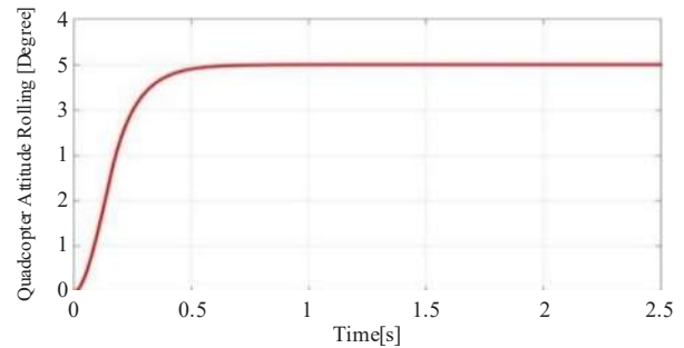
FIG. 4. ROLL RESPONSE
