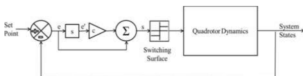
FIG. 2. BLOCK DIAGRAM OF SMC
