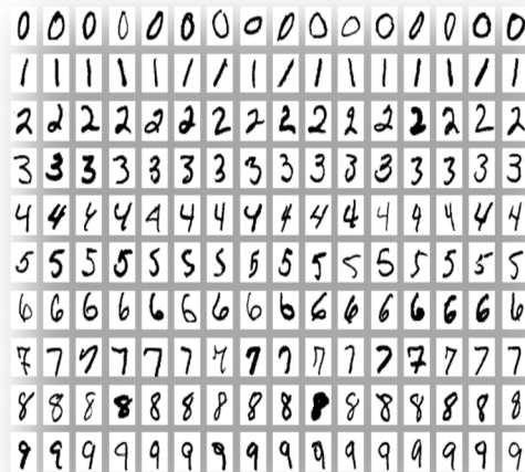
FIG 1: MNIST DATASET
